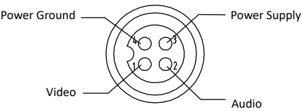
Figure 2-2 Interfaces of Aviation Plug
