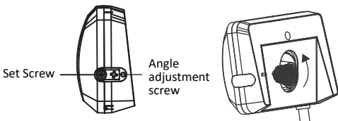
Figure 3-4 Adjust and Fix the Camera Angle
