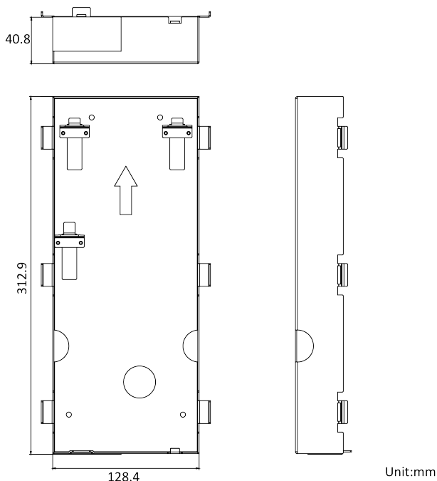
Figure 3-6 Gang Box
