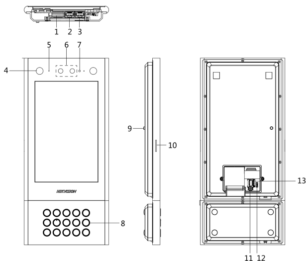
Figure 1-2 Door Station with Keypad Module
