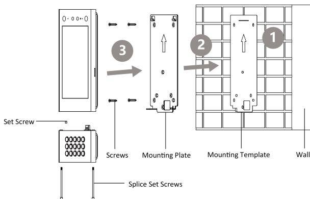
Figure 3-7 Surface Mounting
