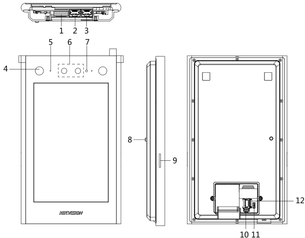
Figure 1-1 Door Station Table 1-1 Appearance Description
