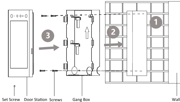
Figure 3-4 Flush Mounting
