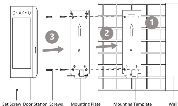
Figure 3-3 Surface Mounting
