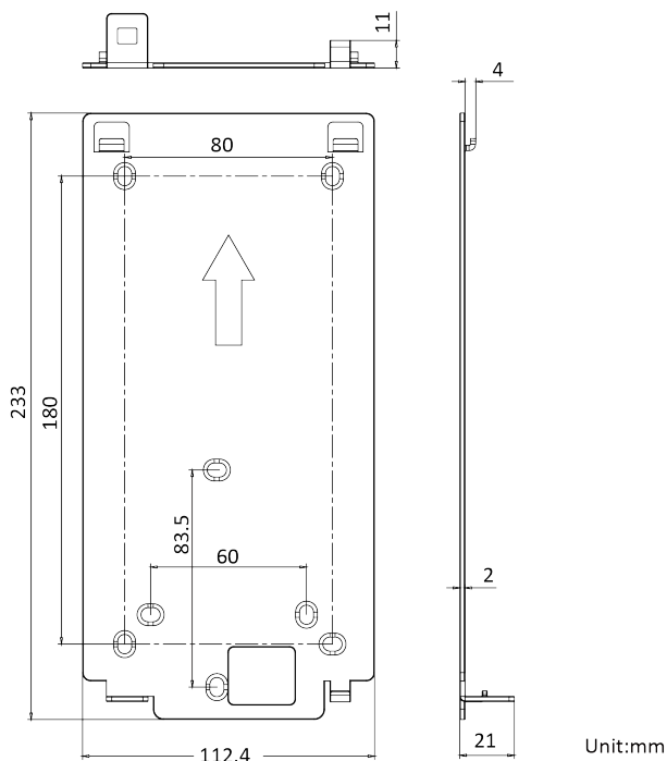
Figure 3-5 Mounting Plate
