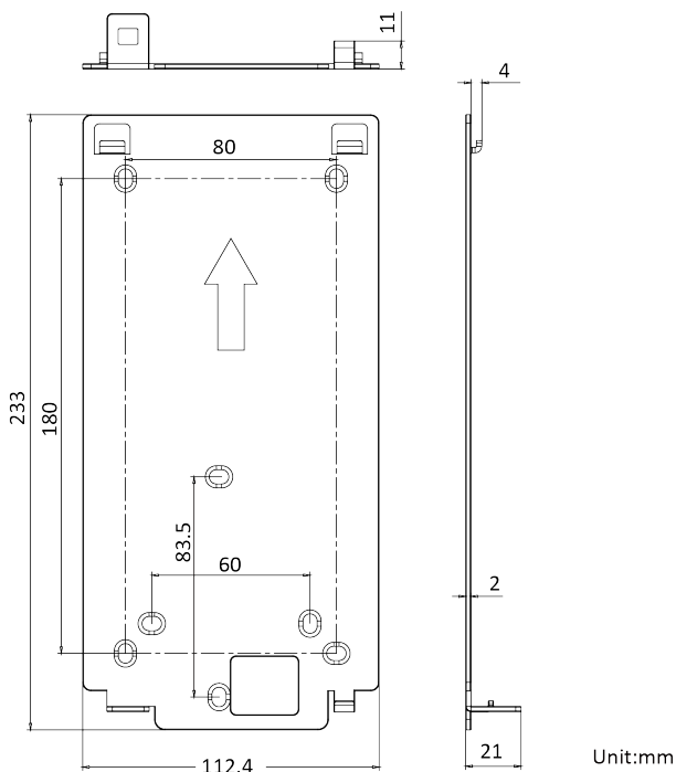
Figure 3-1 Mounting Plate
