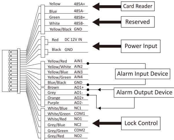
Figure 2-1 Terminal and Wiring Description
