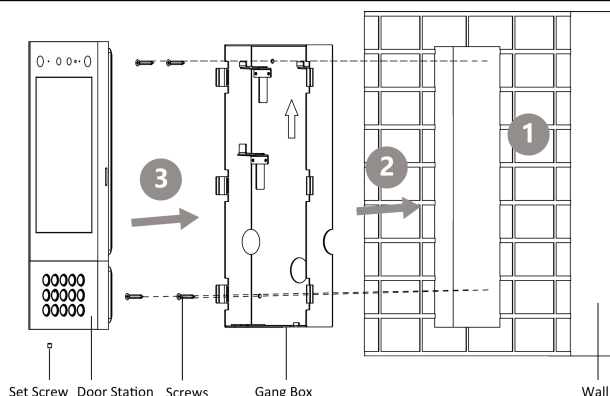
Figure 3-8 Flush Mounting
