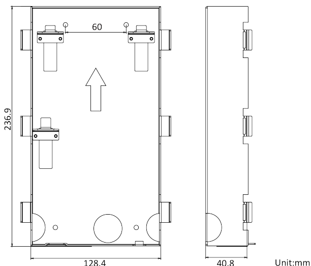
Figure 3-2 Gang Box
