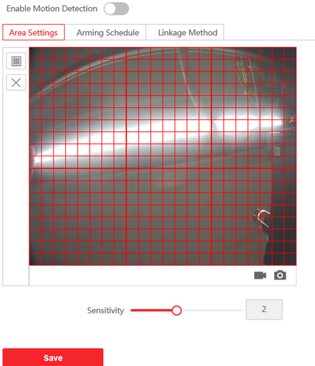
Figure 5-17 Motion Detection
