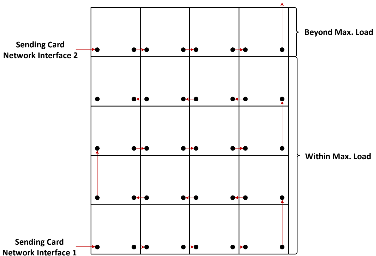
Figure 3-10 Network Cables Connection Between Cabinets
