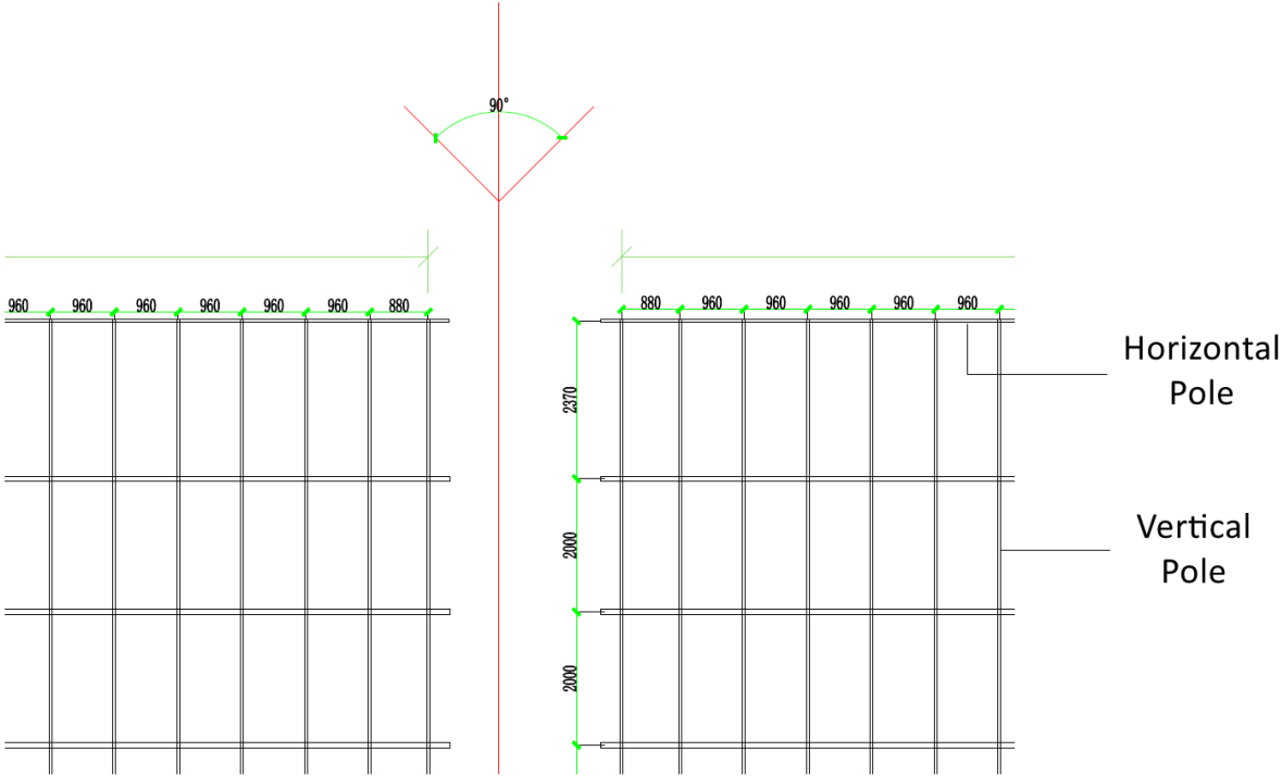
Figure 2-2 Rack Frame (Front View)
