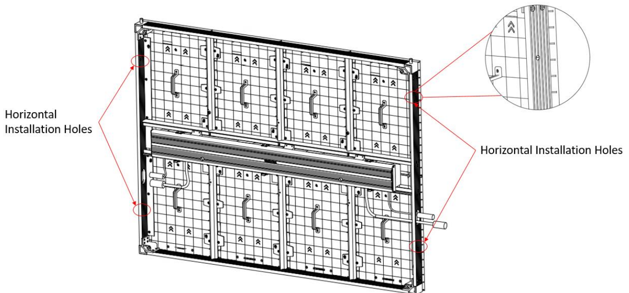
Figure 3-2 Cabinet Frame Locating 2 (Rear)
