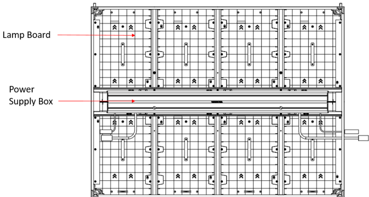
Figure 1-1 Cabinet Overview (Rear)
