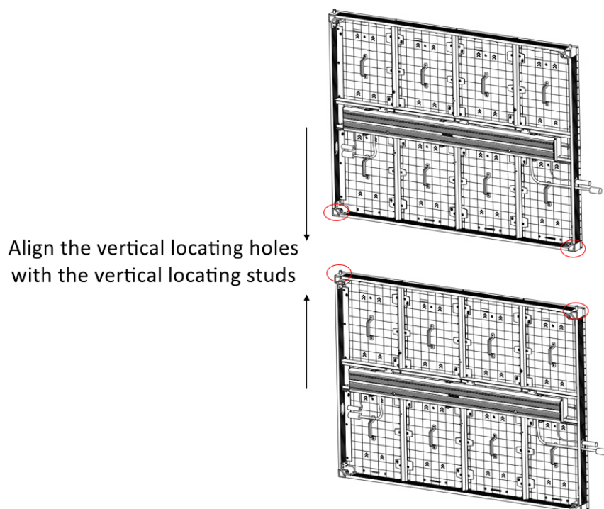
Figure 3-5 Align the Upper Cabinet with the Lower Cabinet
