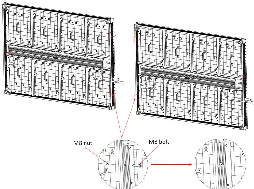
Figure 3-4 Stitch Adjacent Cabinet Frames Horizontally
