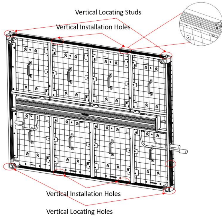
Figure 3-1 Cabinet Frame Locating 1 (Rear)
