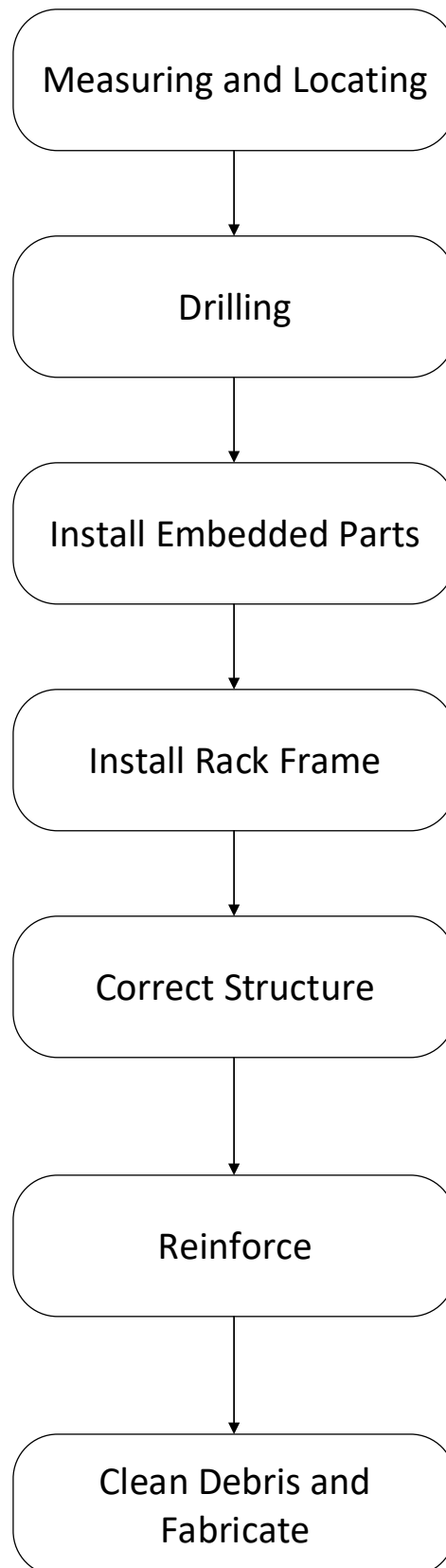
Figure 2-1 Rack Installation Flowchart
