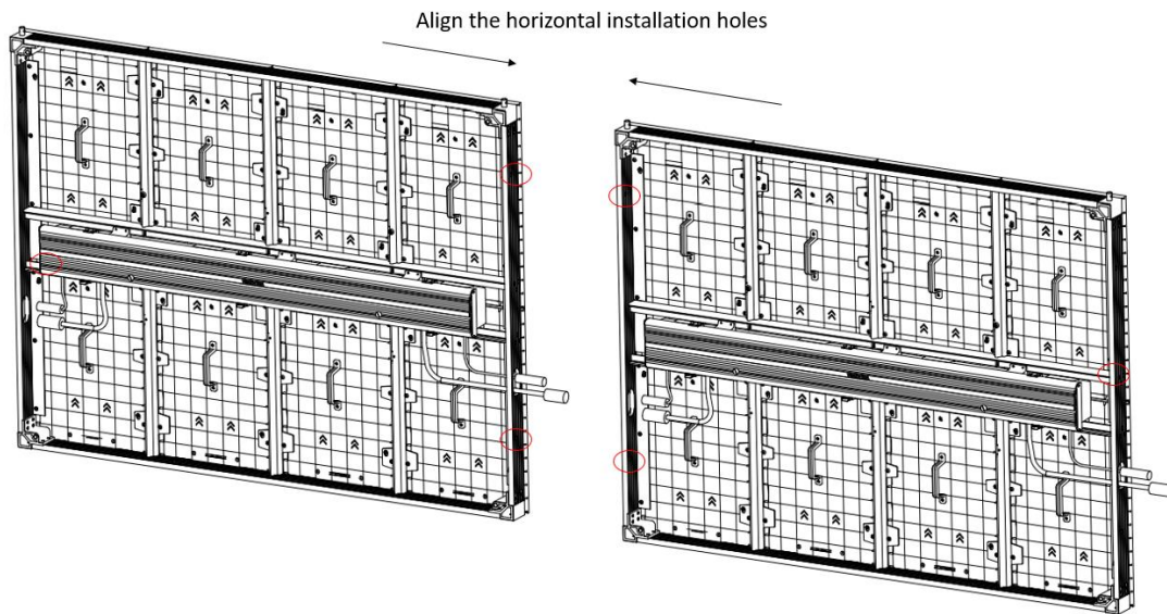
Figure 3-3 Align Two Horizontal Installation Holes
