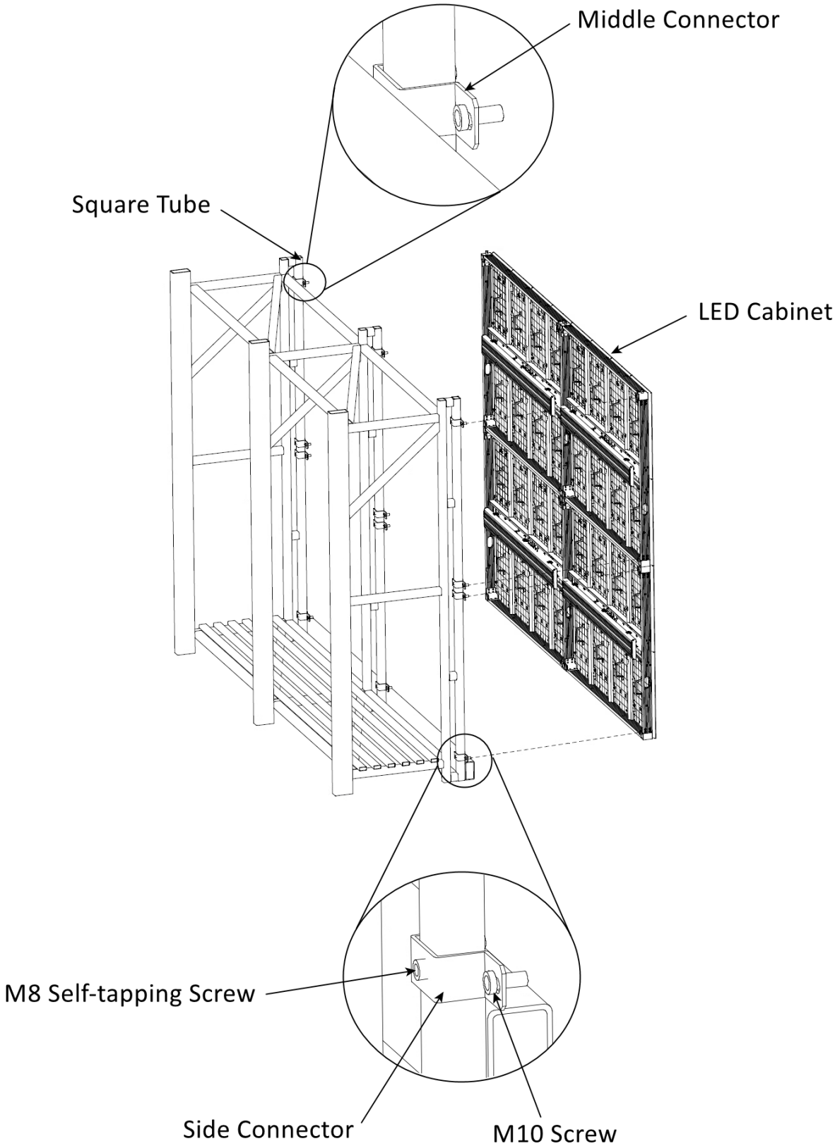
Figure 3-11 Install the Cabinets onto the Rack
