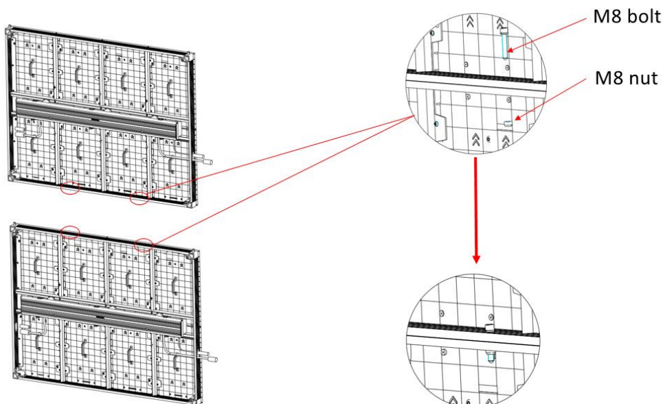
Figure 3-6 Stitch Adjacent Cabinet Frames Vertically
