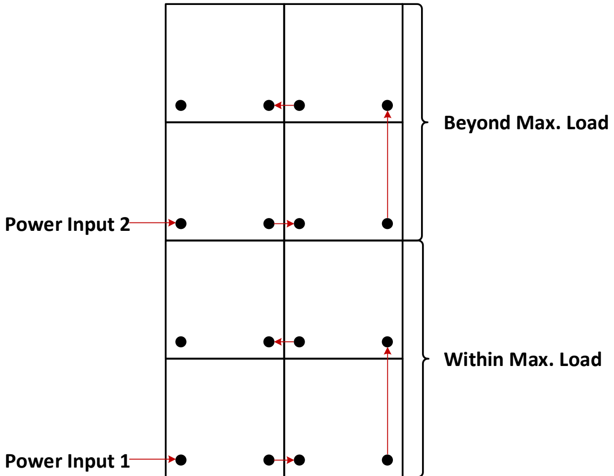
Figure 3-8 Power Cords Connection Between Cabinets
