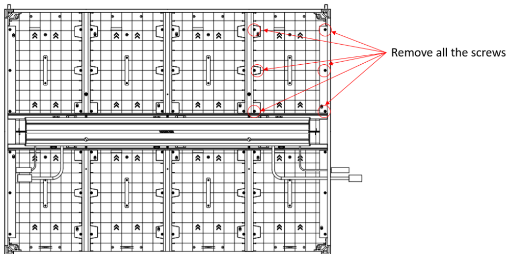
Figure 3-13 Remove All the Screws
