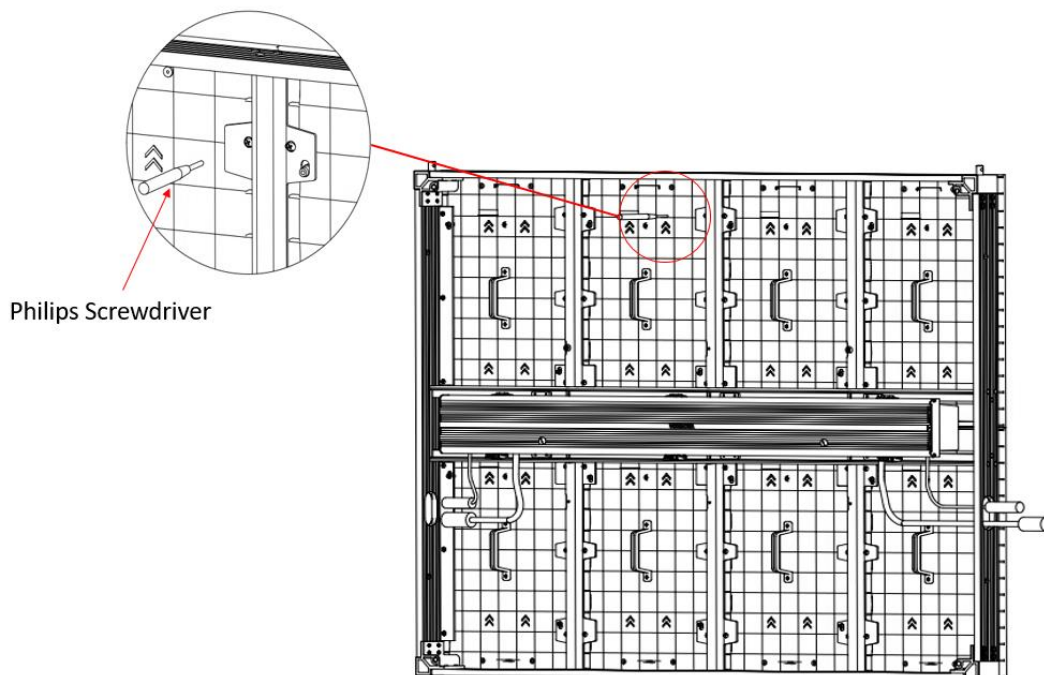
Figure 3-12 Disassemble Lamp Board with Philips screwdriver
