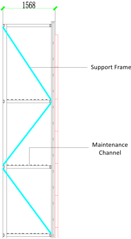
Figure 2-2 Rack Frame (Front View)
