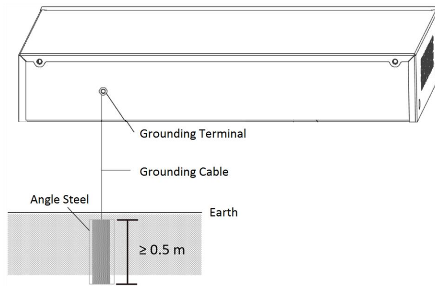
Figure 3-2 Grounding with Angle Steel
