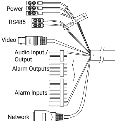
Figure 1-1 Cables I
